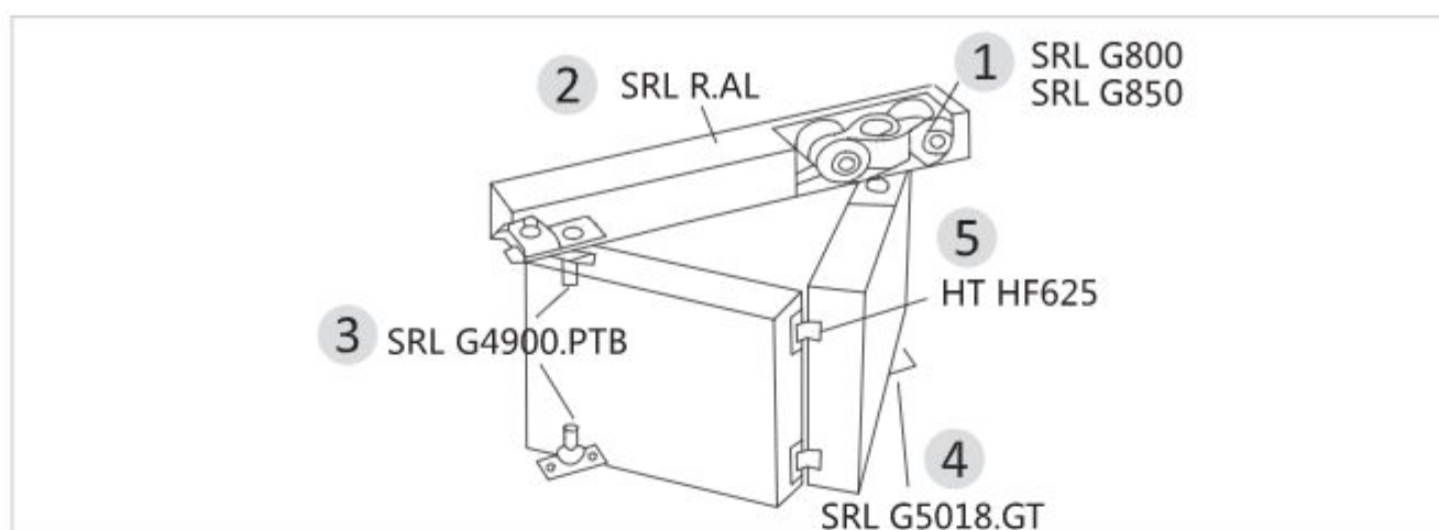
Folding Sliding Door Fittings
