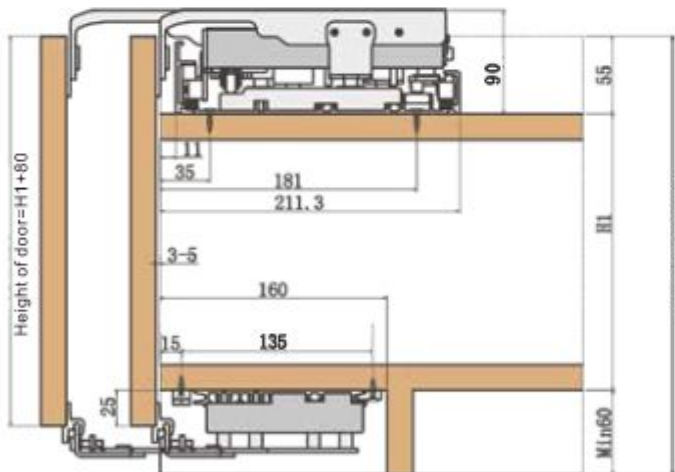
Thickness of door 18-45mm(Handle included)
